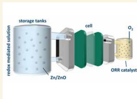
Figure 3: Illustration of a zinc-air battery (not to scale).
