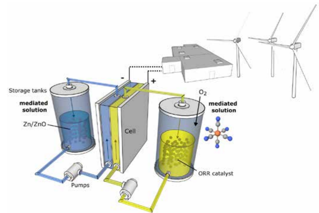
Figure 4: Illustration of a flow battery connected to grid and renewable energy
