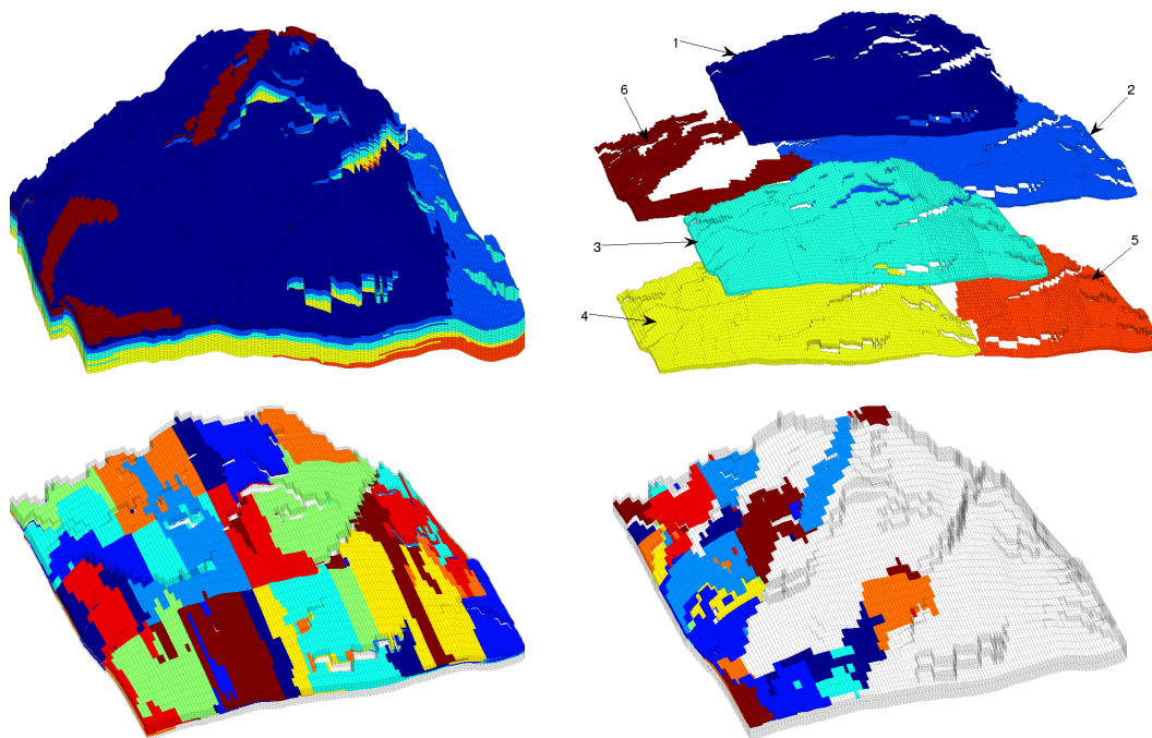
FIGURE 5. Flow-based coarsening of a model faulted SAIGUP model. The upper-left plot shows the structural model. The upper-right plot shows the six saturation regions. The lower plots show the coarse-grid blocks in saturation regions three and six, respectively.
