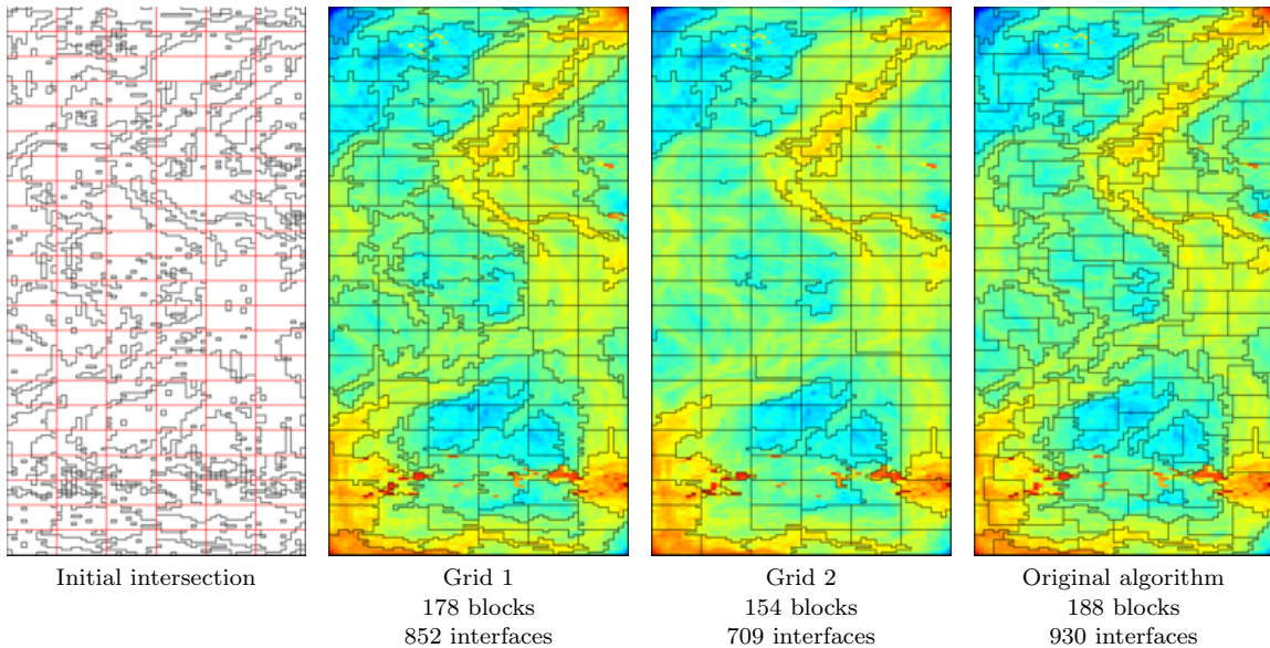
FIGURE 3. Nonuniformly coarsened grids for Layer 1 of Model 2 from SPE10. The leftmost plot outlines the intersection of the initial partitioning, where red lines represent the a priori partitioning and black lines the partitioning into bins. Grid 1 is generated with 10 initial bins and Grid 2 with the number of bins adapted to the flow, and for both we used coarsening parameters N_L=25 , N_U=125 and a uniform 6 \times 22 a priori partitioning. The rightmost plot shows the grid generated by the original algorithm with parameters N_L = 15 , N_U = 75 and a 9-point neighbourhood relation. All three grids are outlined on top of the logarithm of the fine-scale velocity field, computed by solving a quarter five-spot problem.
