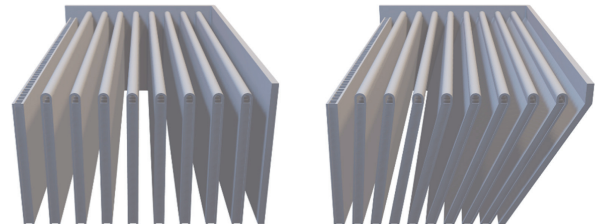
Straight plate-type concept (left) and variable geometry plate-type concept (right).
