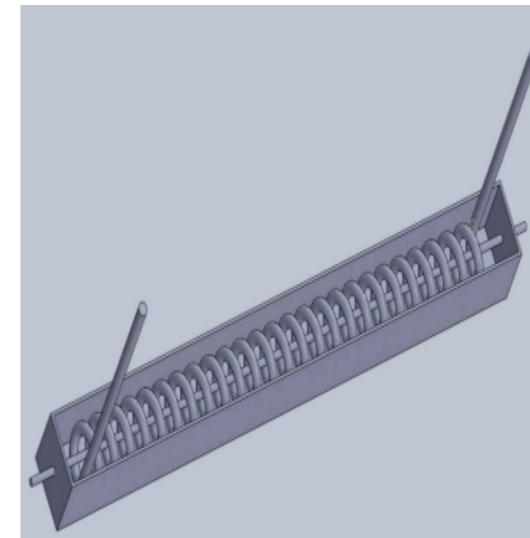
Test section for heat transfer investigation of small tubes.
