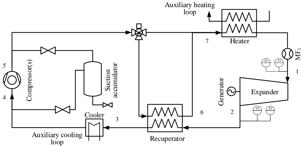
Figure 1: Process flow diagram of the EXPAND test rig.
