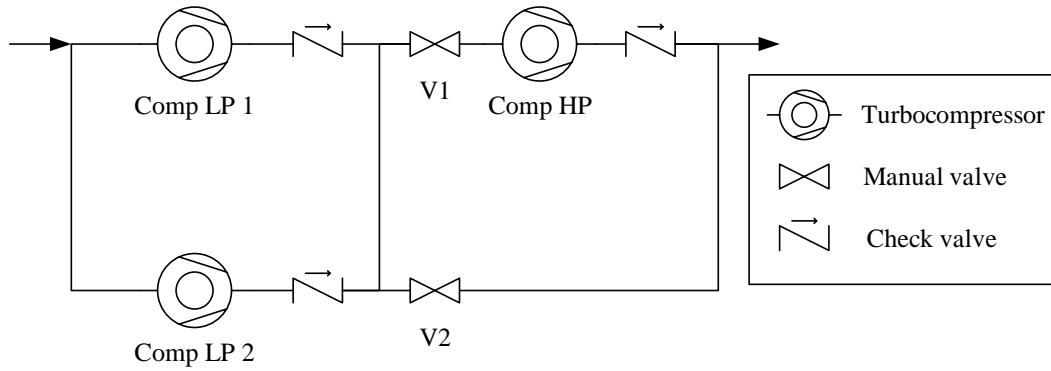
Figure 4: Turbocompressor arrangement used in EXPAND. In the low pressure lift–high mass flow rate configuration Comp LP1 and Comp LP2 are ON and the combined mass flow bypasses Comp HP (V1 is closed and V2 is open). In the high pressure lift–low mass flow rate configuration either Comp LP1 or Comp LP2 is ON and the pressure ratio is further increased by Comp HP (V1 is open and V2 is closed).
