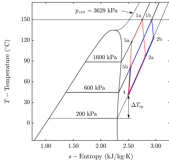
Figure 3: T - s diagram of the test rig for the case of isobutane operating with a pressure ratio of 3 (b) and with a pressure ratio of 8 (a)
