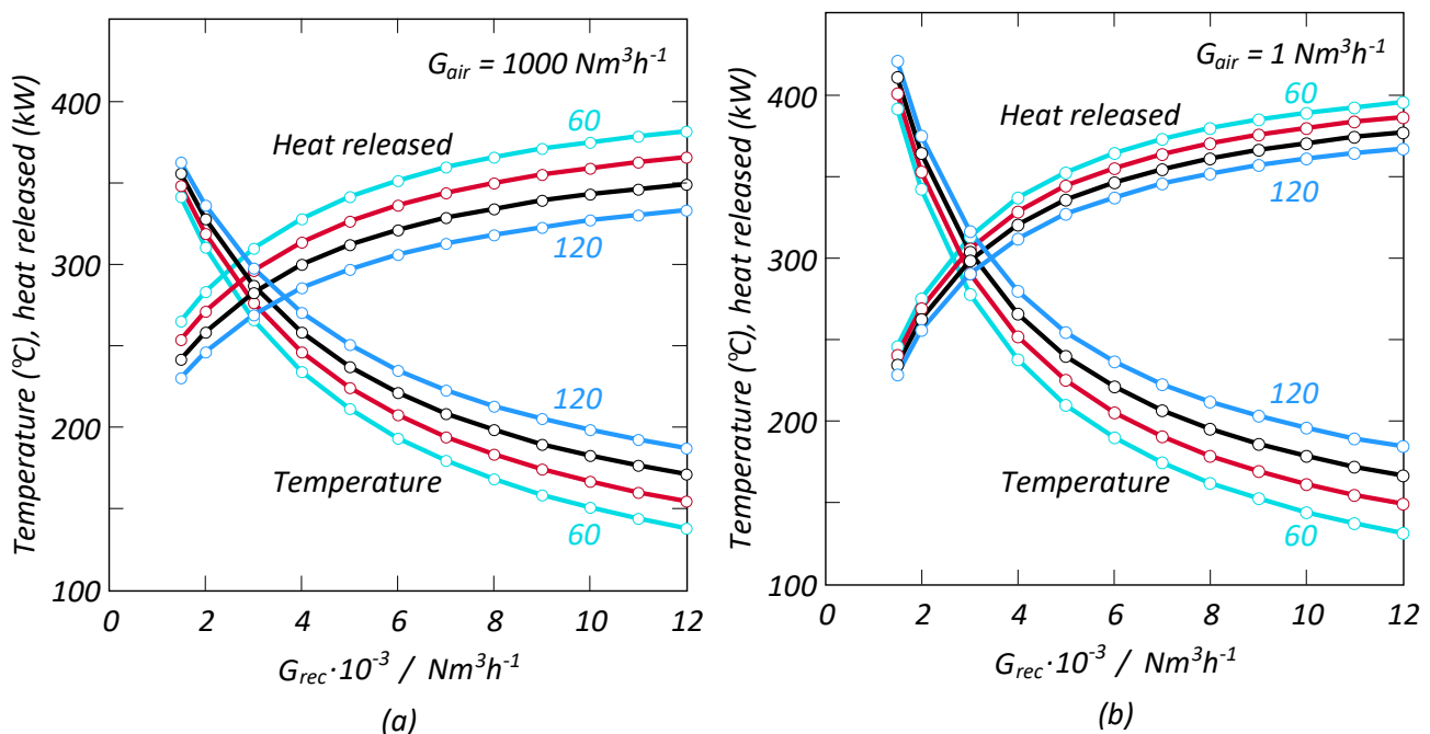
Figure 6. Temperature above the crust and heat released by cooling the flue gas down to the temperatures indicated in the figure as a function of the amount of recycled gas. Calculated with different amounts of air, a): 1000 Nm 3 h -1 , b): 1 Nm 3 h -1 .
