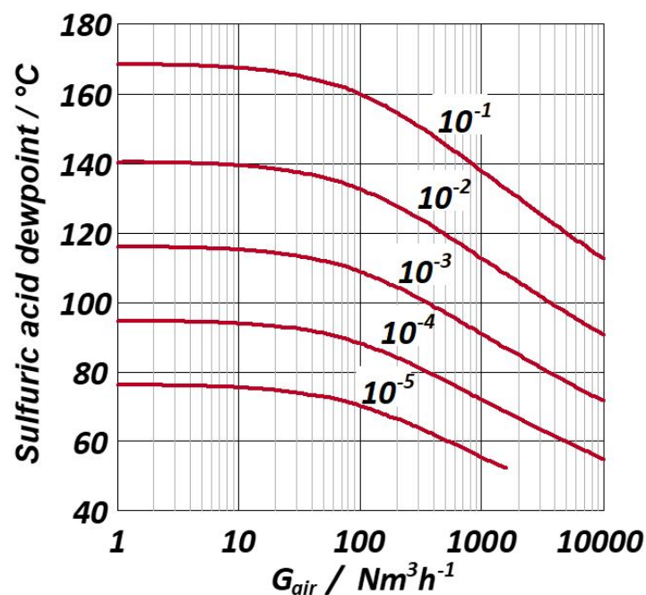
Figure 4. Sulfuric acid dew point as a function of the air draught, calculated as the average of three equations. Same gas composition as in Figure 3. The numbers in the figure represent the ratio between \text{SO}_3 and \text{SO}_2 in the flue gas. The Okkes and Badger equation is out of range at very low concentration of \text{SO}_3 .
