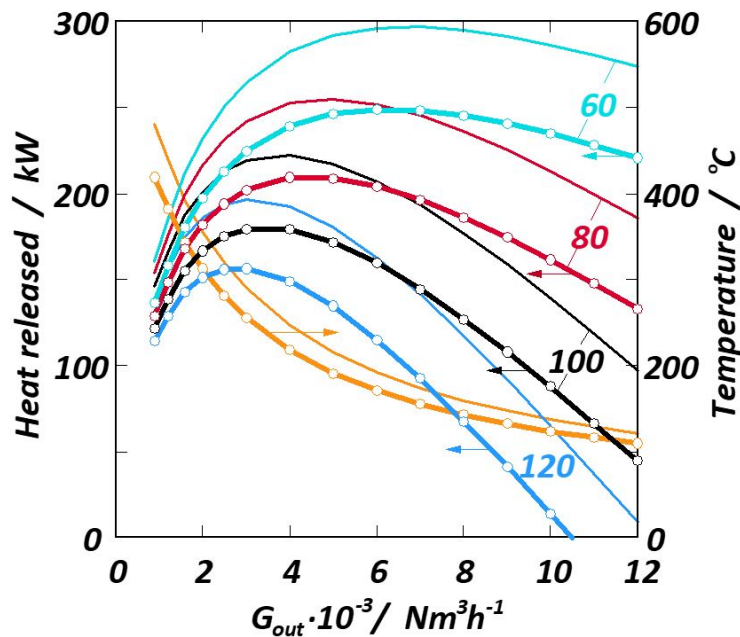
Figure 5. Temperature above crust and heat released by cooling the flue gas down to the temperatures indicated in the figure. Thick lines: No heat from oxidation of CO to CO 2 , Thin lines: Including heat from oxidation of all CO.
