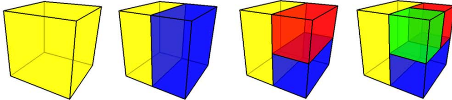
Figure 6: Construction of a 3 dimensional LR-mesh in parameter space.
