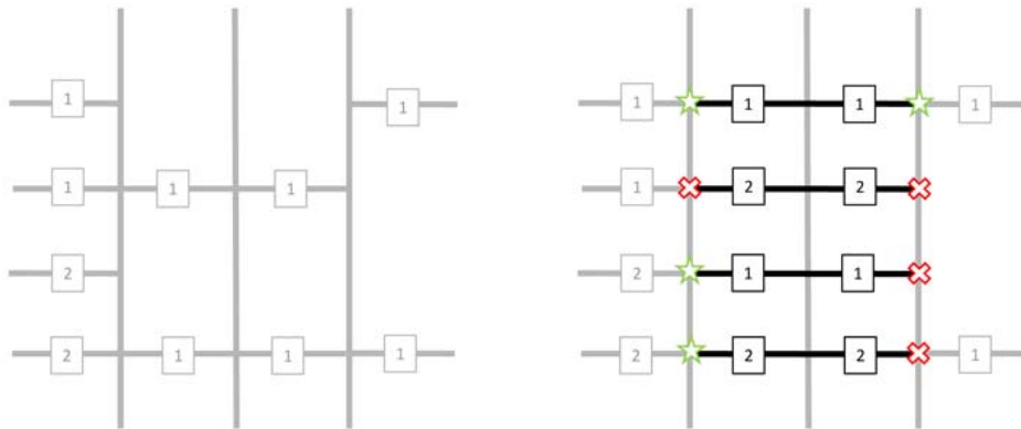
Figure 11: This illustration shows attachment of 4 inserted horizontal segments. Only mesh-rectangles in the same hyperplane as the inserted mesh-rectangle have to be considered and vertical multiplicities are irrelevant for this example. Going from top to bottom the first segment has multiplicity 1 and is attached at both ends. The next segment has multiplicity 2 while there is no horizontal neighboring segment to the right and the one to the left has multiplicity one. This segment is not attached at either end. The third and fourth segments are both attached at the left end, but not at the right.
