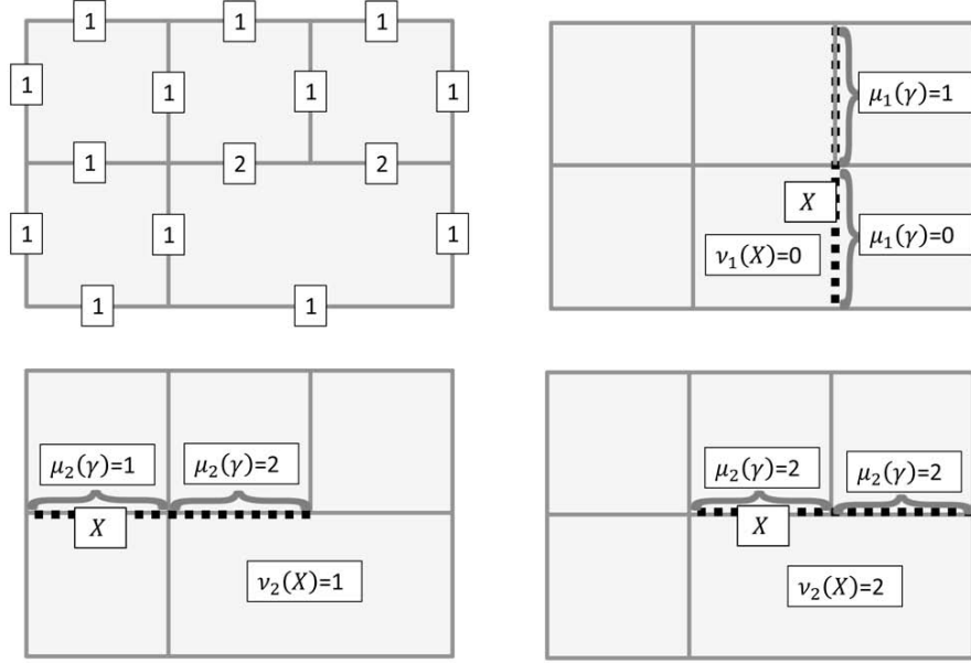
Figure 7: A \mu -extended box-mesh, and three examples of sets X (dotted) and the resulting value of \nu_k(X) .
