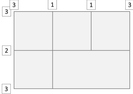
Figure 10: A biquadratic case where the continuity across internal vertical edges is C^1 , e.g., r_1 = 1 , and the continuity across internal horizontal edges is C^0 , e.g., r_2 = 0 . We find \dim(\mathbb{S}_{\mathbf{p}}(\mathcal{M}, \mu)) = 3 \times 3F_2 - 3 \times 1F_1^h - 2 \times 3F_1^v + 2 \times 1F_0 = 22 based on the counting: F_2 = 5 , F_1^h = 3 , F_1^v = 3 , and F_0 = 2 .
