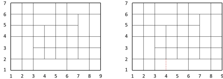
Figure 14: Linear dependence of bi-quadratic LR B-splines. In this LR-mesh all mesh-rectangles have multiplicity 1.
