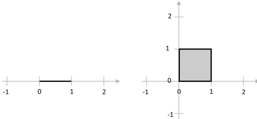
Figure 1: In the Figure to the left there are two (0, 1) -boxes (points/mesh-rectangles) \{0\} and \{1\} , and one (1, 1) -box (element) [0, 1] . In the Figure to the right there are four (0, 2) -boxes (points) (0, 0) , (1, 0) , (0, 1) and (1, 1) , four (1, 2) -boxes (line segments/mesh-rectangles) [0, 1] \times \{0\} , \{0\} \times [0, 1] , [0, 1] \times \{1\} , and \{1\} \times [0, 1] , and one (2, 2) -box (element) [0, 1] \times [0, 1] .
