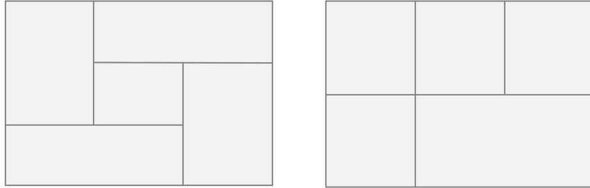
Figure 5: A box-mesh (left) and an LR-mesh (right)
