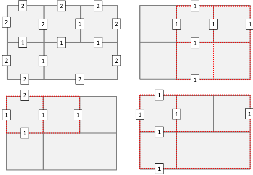
Figure 8: A \mu -extended box-mesh \mathcal{M} at the top left, and 3 examples of bilinear B-splines and their relation to \mathcal{M} . The B-spline indicated by the knotline multiplicities at the top to the right does not have support in \mathcal{M} since a part of a knotline of the B-spline is not present in \mathcal{M} . The two examples below has support in \mathcal{M} , but only the B-spline to the right has minimal support in \mathcal{M} . In the B-spline to the left the internal vertical knotline has lower multiplicity than the corresponding mesh-rectangle in \mathcal{M} .
