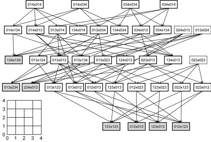
Figure 15: An LR-mesh and corresponding bilinear LR-graph .
