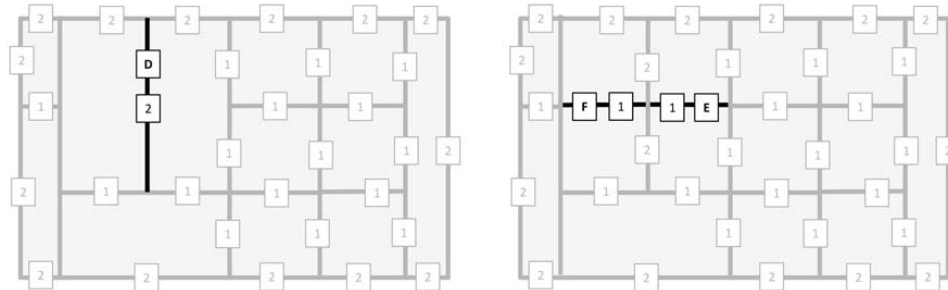
Figure 13: The illustration shows refinements related to mesh-rectangles of multiplicity higher than 1, and to the filling of gaps between already existing mesh-rectangles. To the left the result of the refinement in Figure 12 with mesh-rectangle D inserted on top of mesh-rectangle C, thus increasing the multiplicity from 1 to 2. To the right we first insert the mesh-rectangle E (mesh-rectangle F has not been inserted yet) that ends in a T-vertex with multiplicity 2. This increases the dimension of the spline space by 2. Then we fill a gap by mesh-rectangle F, that further increases the dimension of the spline space by 2.
