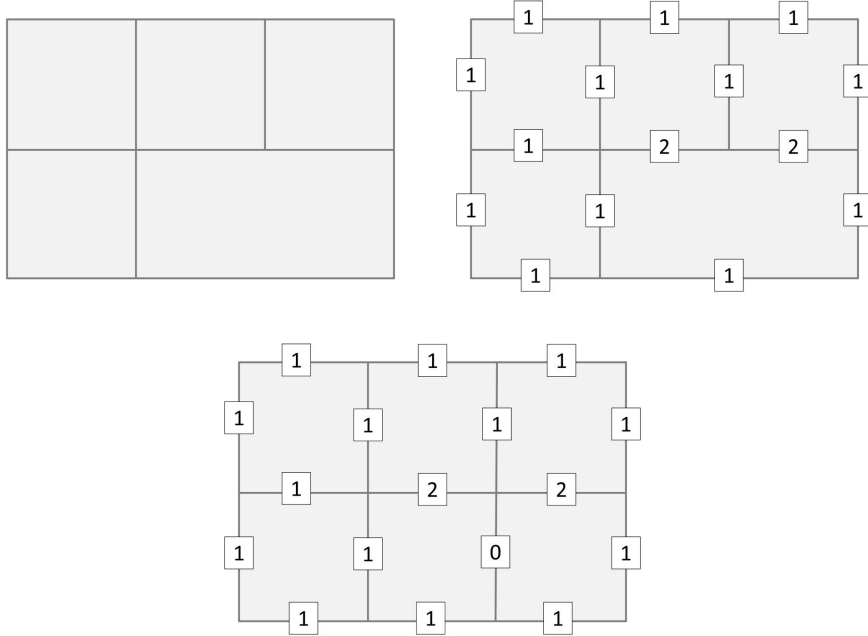
Figure 3: A box-mesh, an example of a \mu -extension, and its tensor-mesh expansion.
