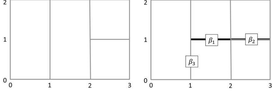
Figure 4: An illustration of the three cases in Definition 2.11. The mesh-rectangle \gamma = [1, 3] \times \{1\} is inserted. The mesh-rectangle \beta_1 = [1, 2] \times \{1\} \subseteq \gamma does not exist from before and is assigned multiplicity 1. On the other hand \beta_2 = [2, 3] \times \{1\} \subseteq \gamma is already present and the multiplicity is increased by one. The third case is illustrated by \beta_3 = \{1\} \times [0, 1] that is a subset of the mesh-rectangle \{1\} \times [0, 2] that existed before \gamma was inserted but that is not a subset of \gamma .
