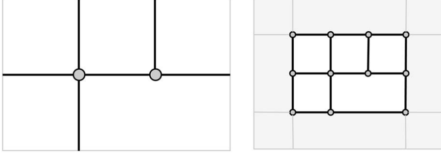
Figure 2: The Figure shows an example of a box partiton \mathcal{E} to the left, \mathcal{E} \cup \Omega^+ to the right, and their lower dimensional boxes.
