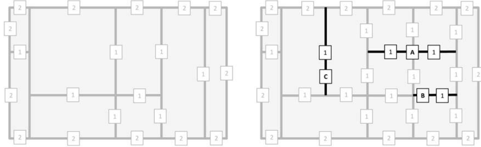
Figure 12: To the left a bi-linear \mu -extended LR-mesh illustrating the 3 cases in Corollary 5.6. The multiplicity is 2 along the boundary, and 1 for interior mesh-rectangles. Mesh-rectangle A has two segments and ends in a T-vertex at both ends; Mesh-rectangle B extends an interior mesh-rectangle by one segment and ends in a T-vertex; Mesh-rectangle C starts from the boundary, and has one segment. Note that extending C to touch the lower boundary would increase the dimension of the spline space by two, and is thus not covered in Corollary 5.6.
